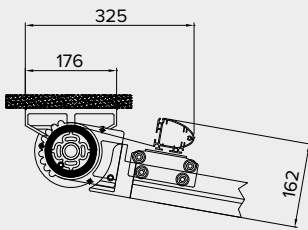
Attacco a soffitto . Ceiling application
