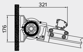
Attacco a parete . Wall application
