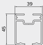
Guide Laterali . Side rail
