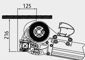
Attacco a soffitto . Ceiling application
