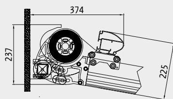
Attacco a parete . Wall application
