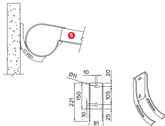
Staffa attacco parete . Wall application bracket 088-902
