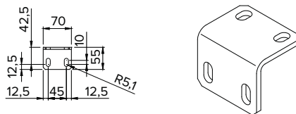
Attacco a spallina . Inside application 088-914
